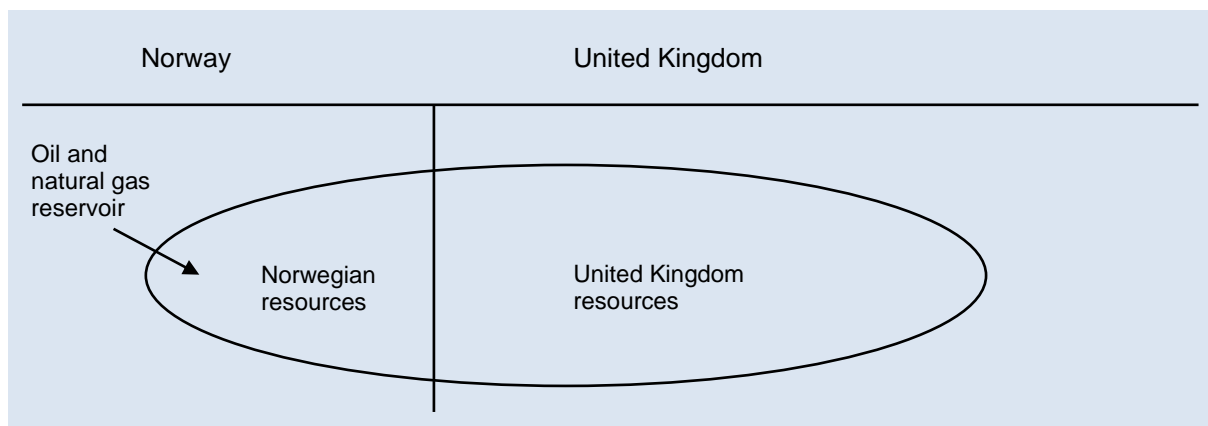
Figure 8.3 Cross border petroleum deposits
